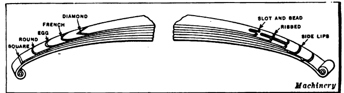
Fig. 3—Varieties of spring plate ends in common use
